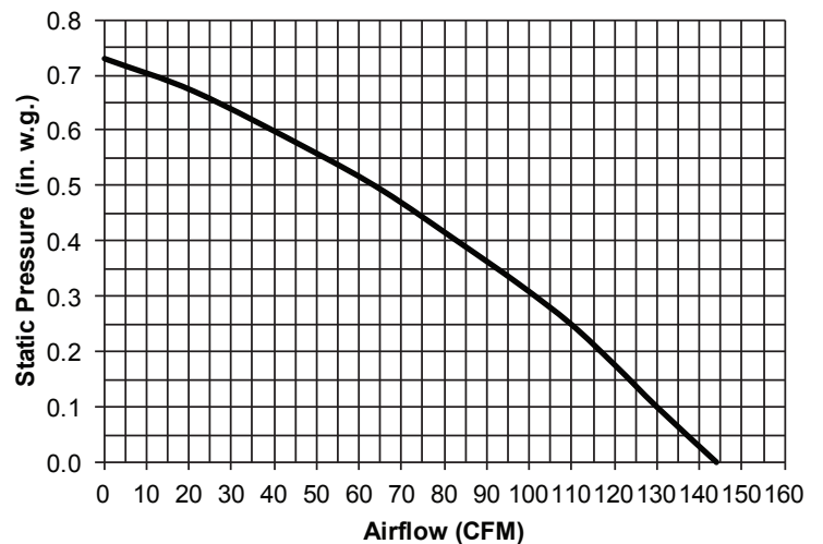
MODEL QT140E - 4" DUCT
